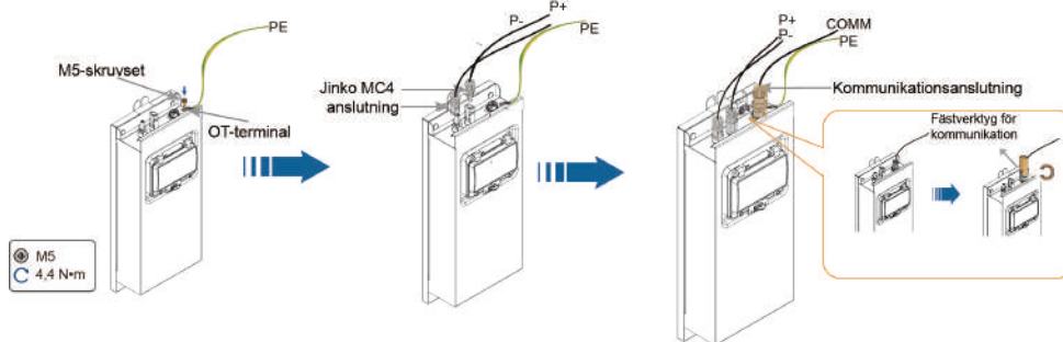
Connection Diagram
